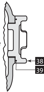
Model 441-57S General Assembly 2" and 3" Models
