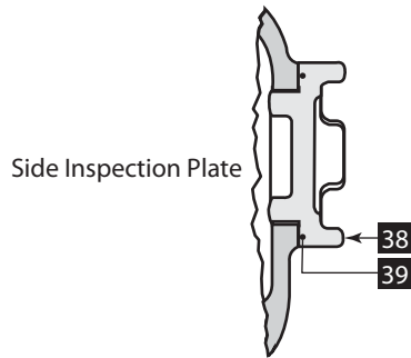
Model 441-57S General Assembly 4" Model
