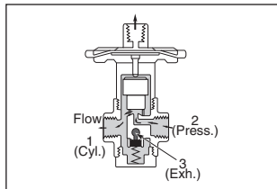
Figure 12A: Normally Open, Operator Exhausted
