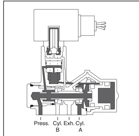
Figure 6A: Four-Way Valve, De-Energized
